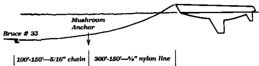
Figure 7 DOUBLE CHAFFING GEAR
